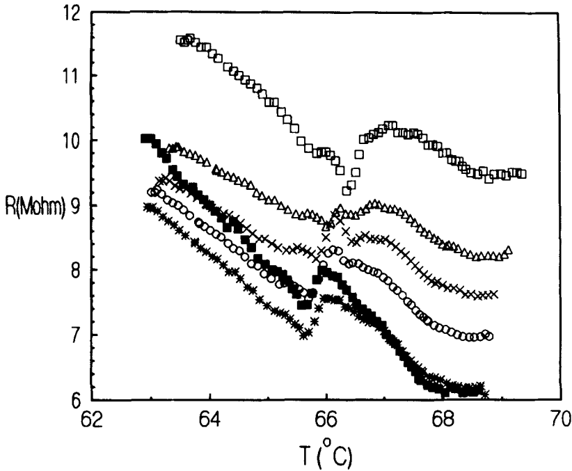
FIGURE 8 Variation of the resistance of 8OCB as a function of temperature at different values of the applied voltage across T_{AN} . The frequency used is 2170 Hz.
