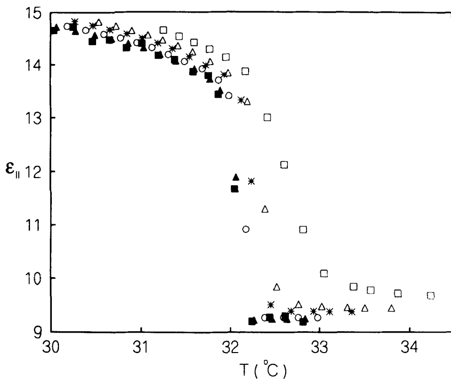
FIGURE 4 Dielectric constant ( \epsilon_{||} ) of 5CB as functions of temperature and voltage across NI transition; frequency of the applied voltage is 2317 Hz. ■ (1.05 V), ▲ (31.8 V), ○ (77.0 V), * (137.0 V), △ (182.8 V), □ (285.5 V).
